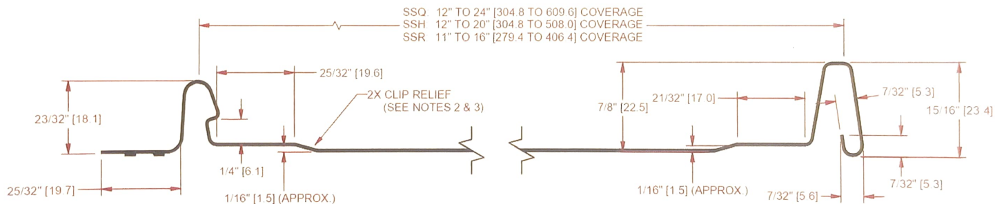
DETAIL A
